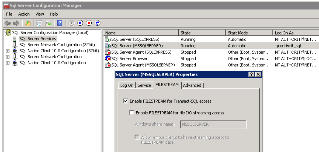
Figure 10 Enabling FILESTREAM
