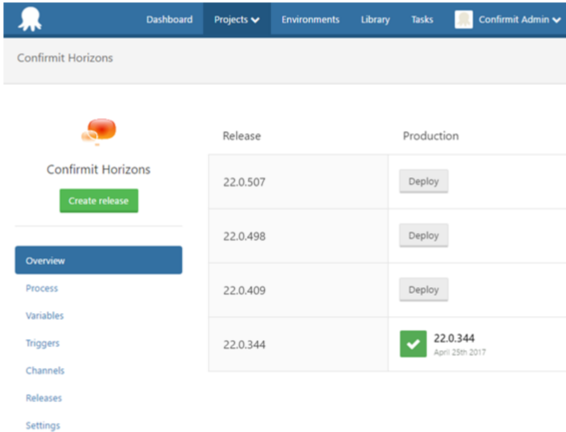
Figure 20 Click Deploy
