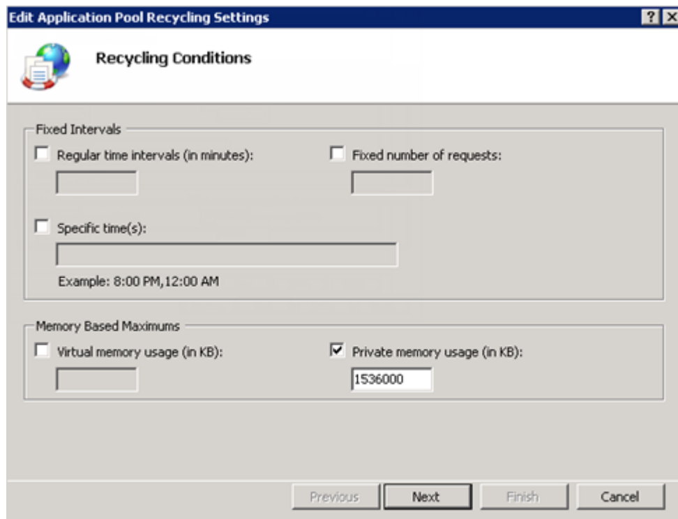
Figure 40 The Recycling Conditions page
