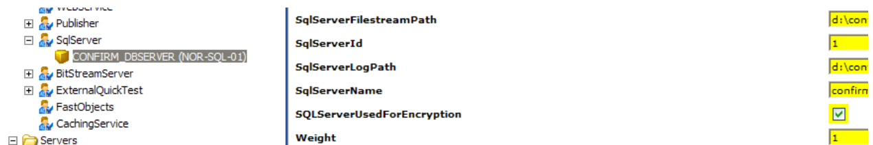
Figure 48 Checking the SqlServerUsedForEncryption checkbox
