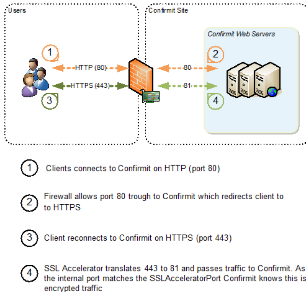
Figure 41 Using Confirmit with a load balancer
