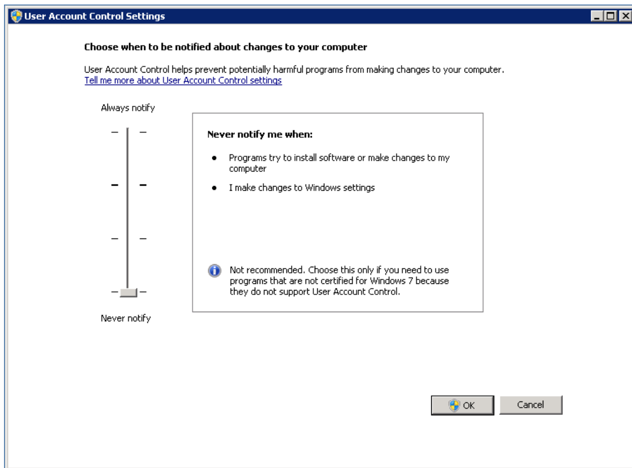
Figure 24 Disabling UAC
