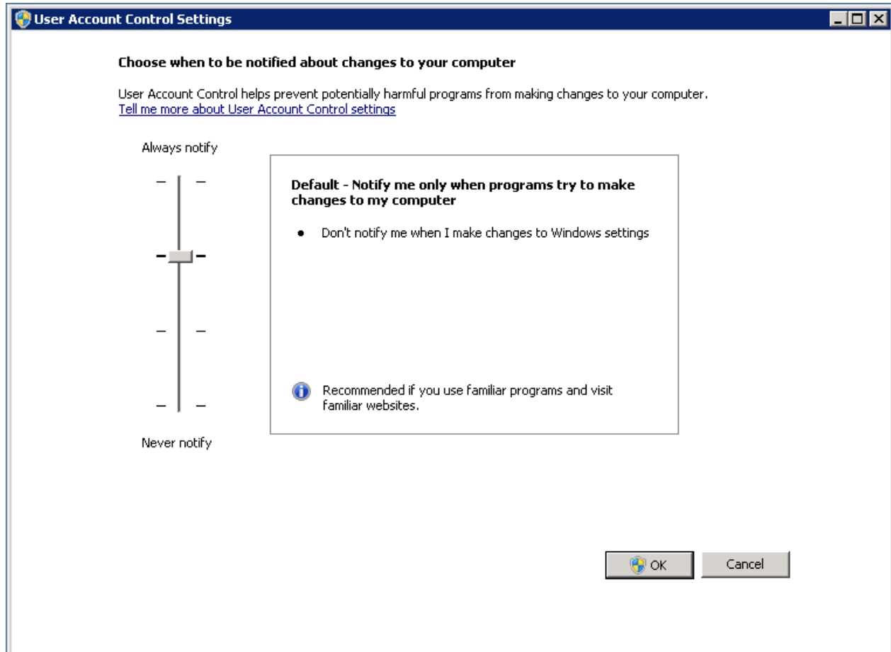
Figure 25 Enabling UAC
