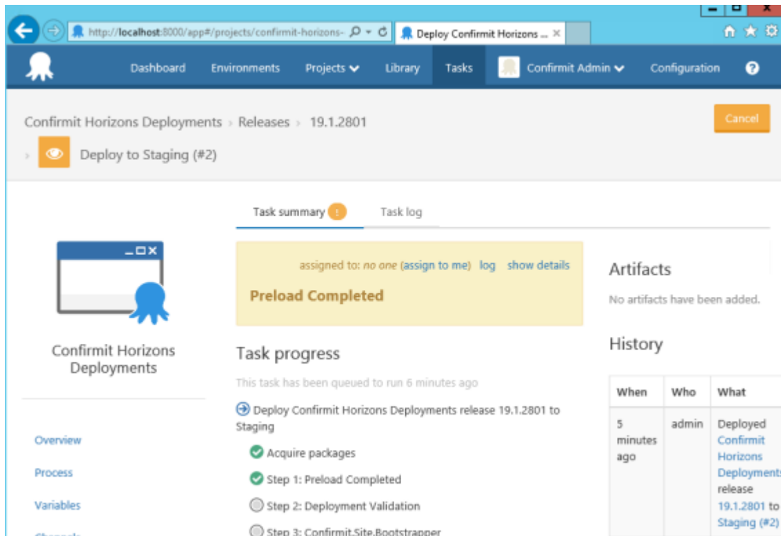
Figure 22 Preload complete
