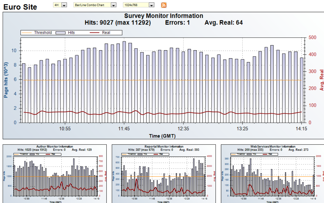
Figure 52 Example of the monitoring utility screen layout
