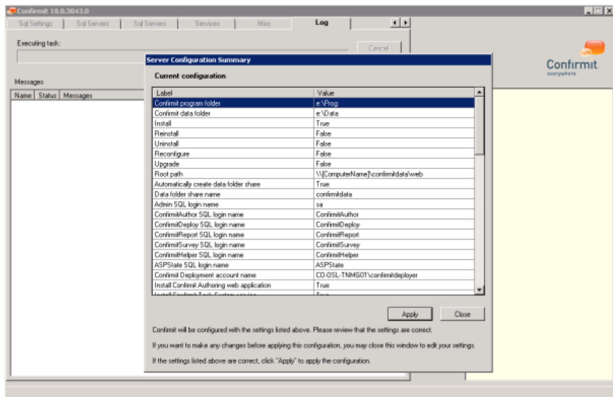
Figure 19 Reviewing the selected settings
