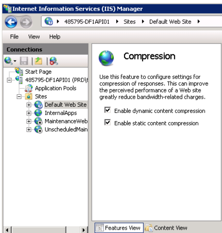
Figure 41 Compression settings for web site
