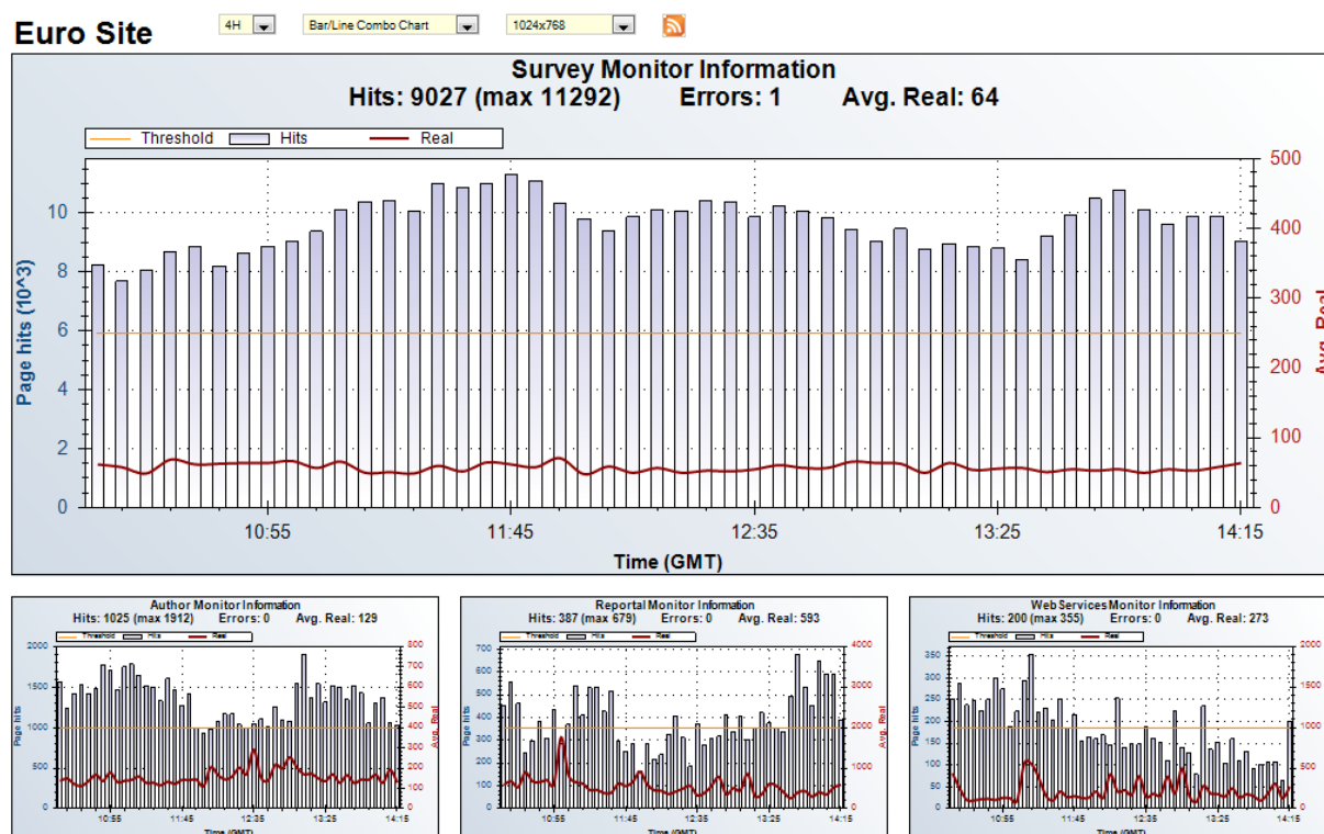
Figure 49 Example of the monitoring utility screen layout
