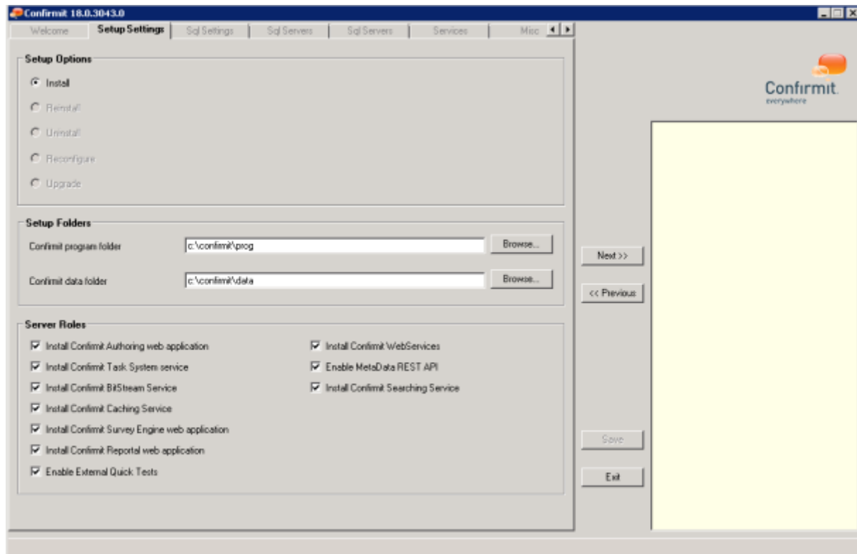
Figure 13 The Destination Folder and Role Selection page
