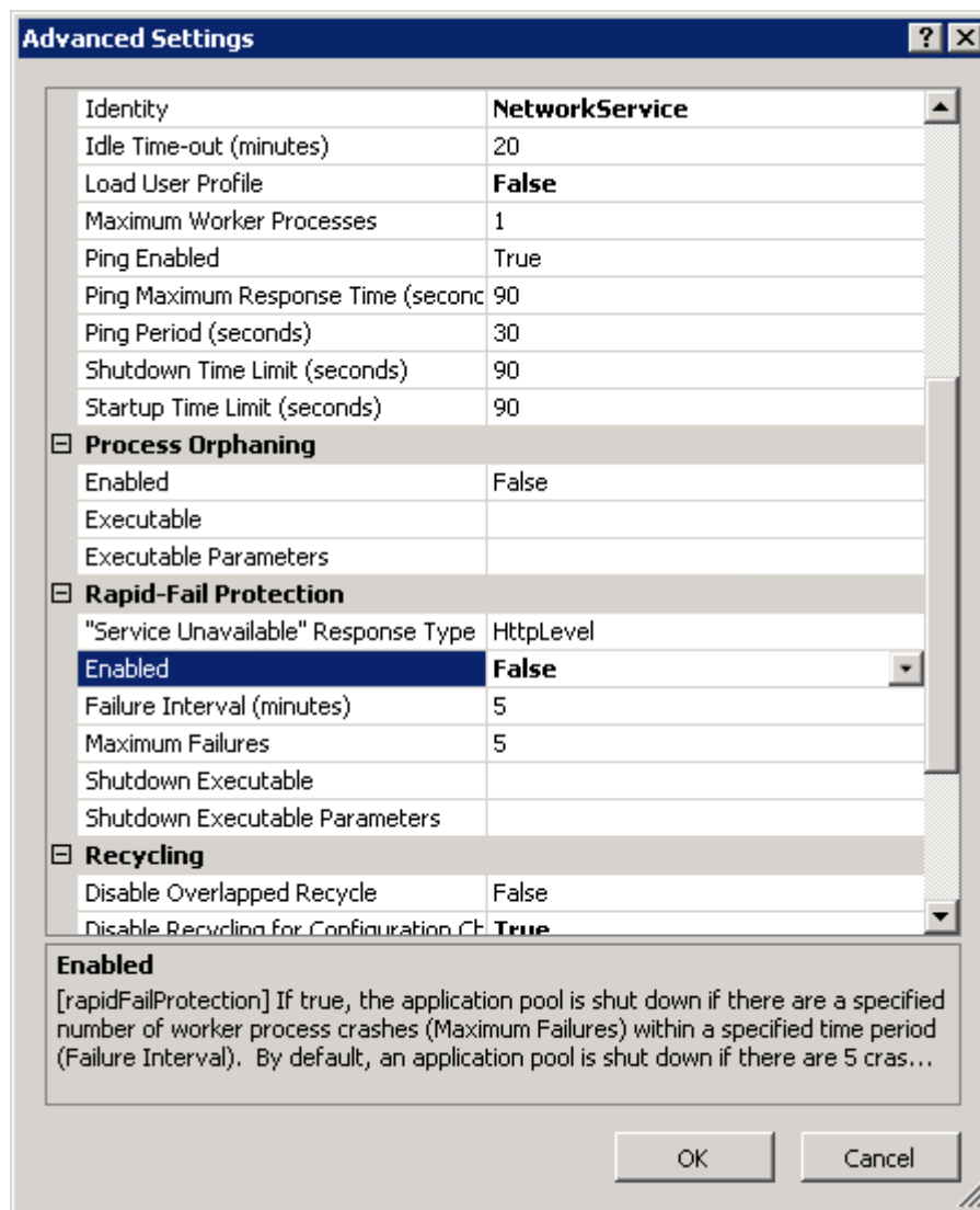
Figure 39 The Advanced Settings page - 2
