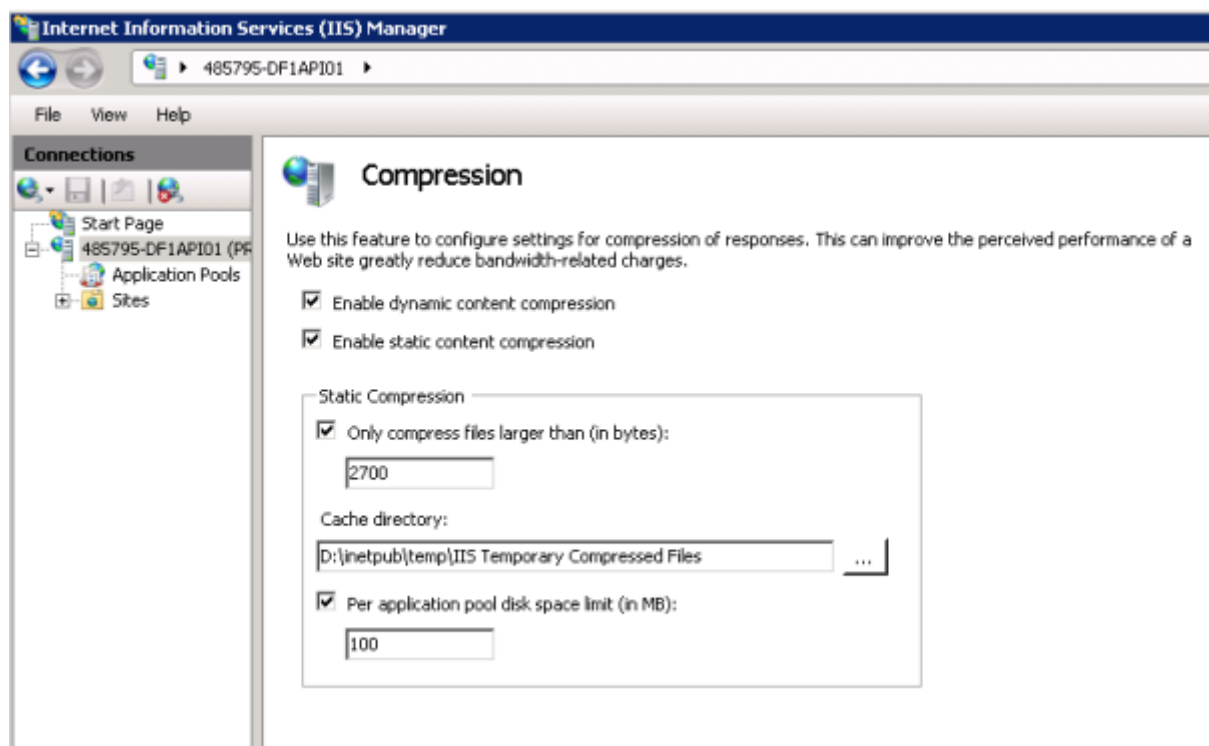
Figure 40 Compression settings for servers
