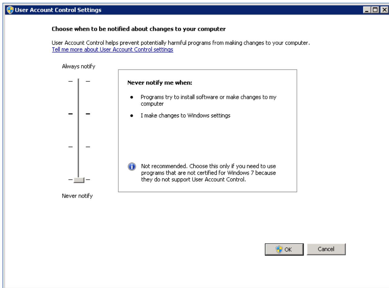
Figure 24 Disabling UAC
