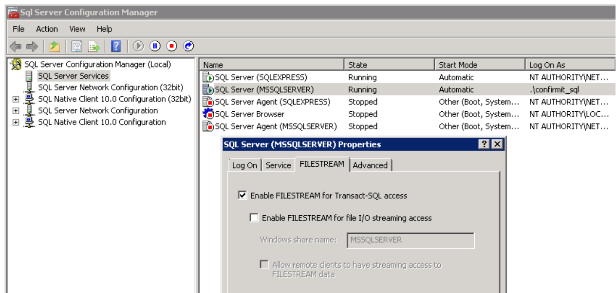
Figure 10 Enabling FILESTREAM
