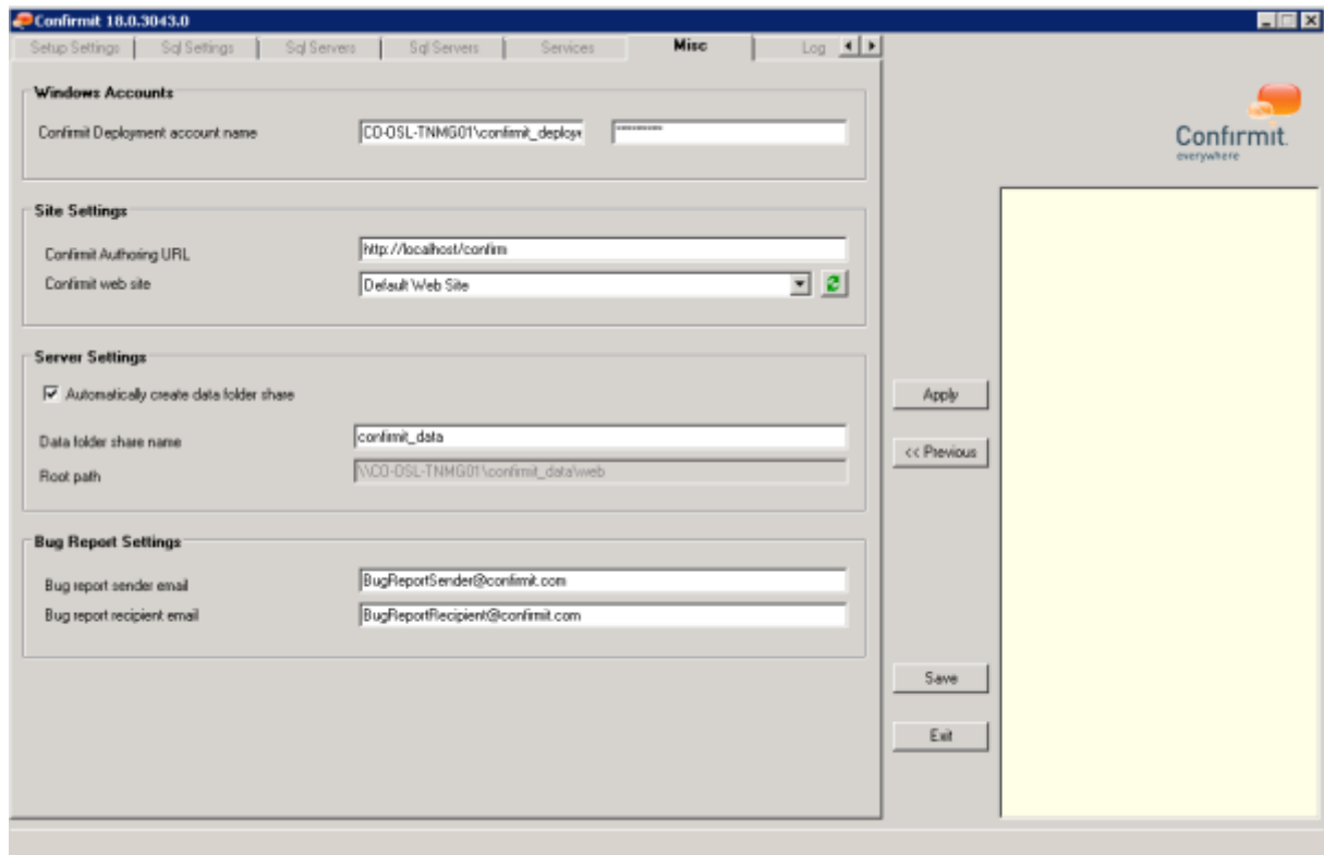
Figure 20 The Miscellaneous page
