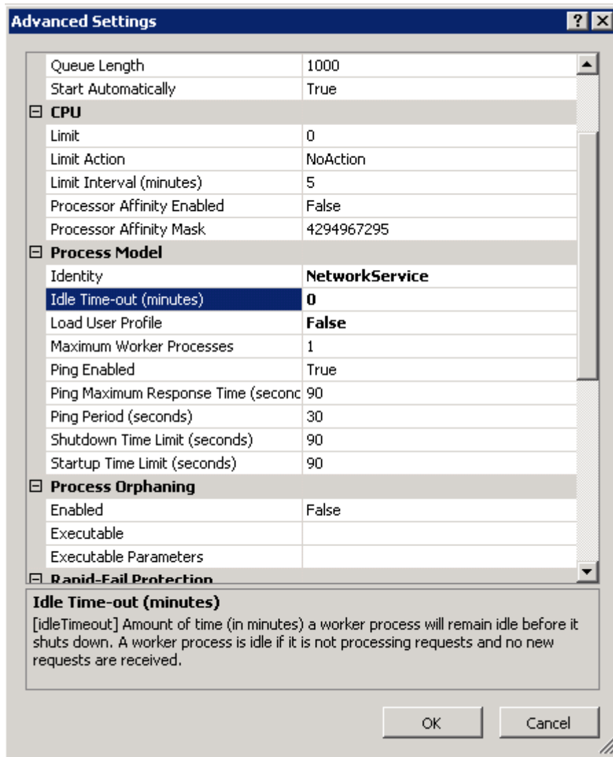
Figure 36 The Advanced Settings page - 1
