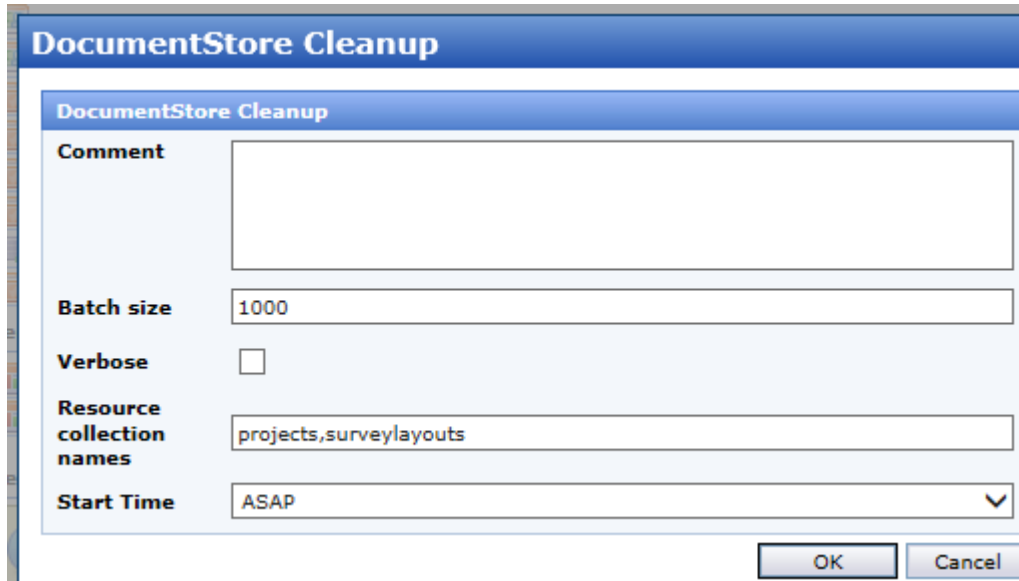
Figure 32 The DocumentStore Cleanup overlay
