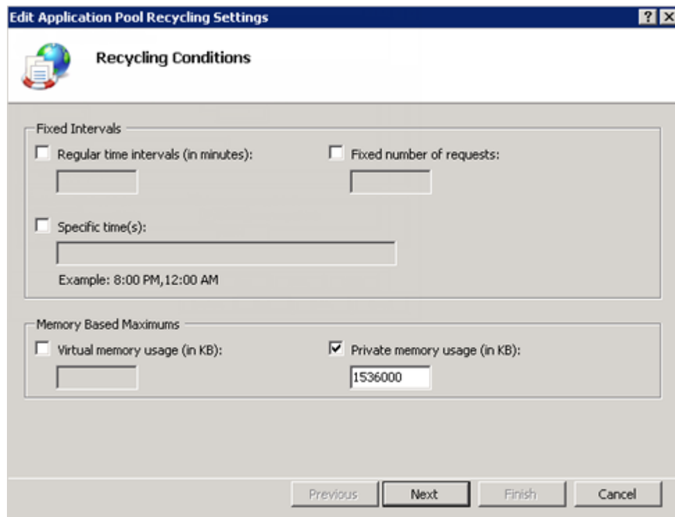
Figure 35 The Recycling Conditions page
