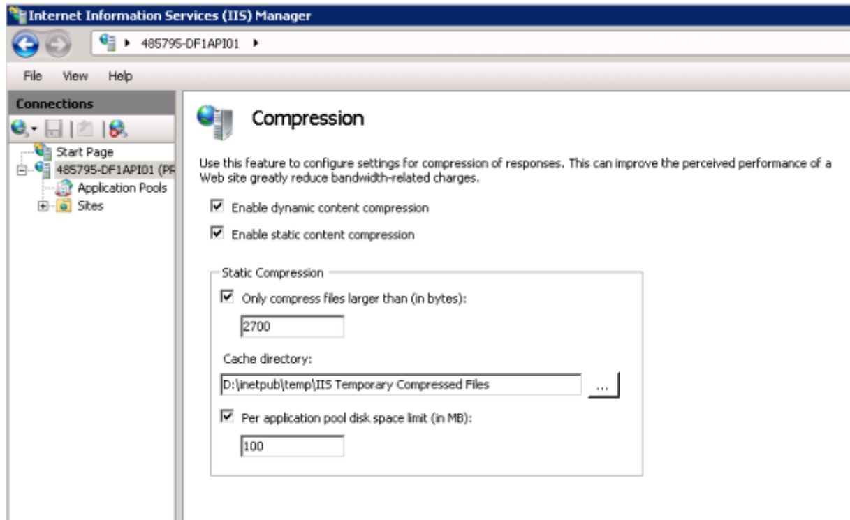
Figure 38 Compression settings for servers
