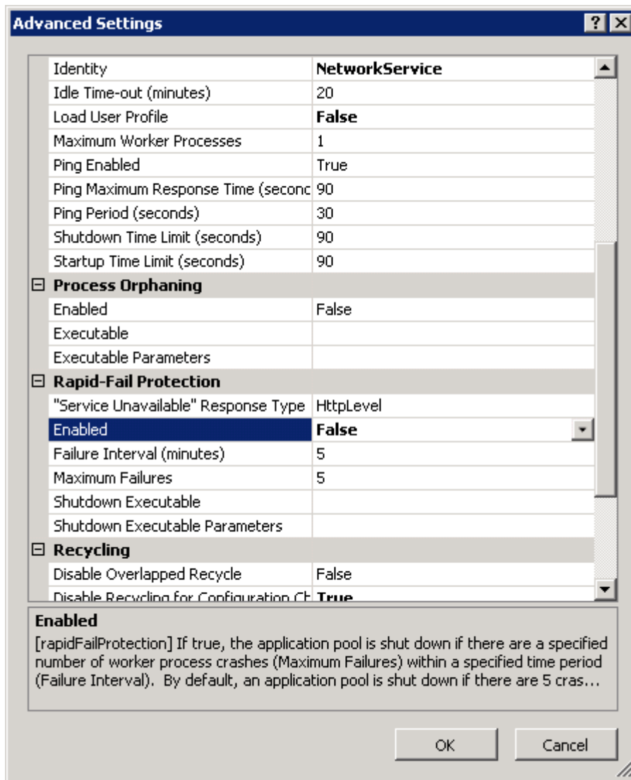
Figure 37 The Advanced Settings page - 2
