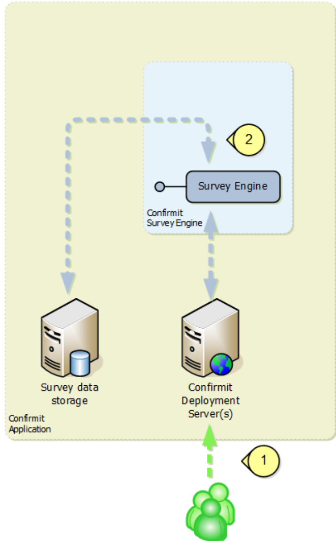
Figure 3 The Confirmit Survey dataflow
