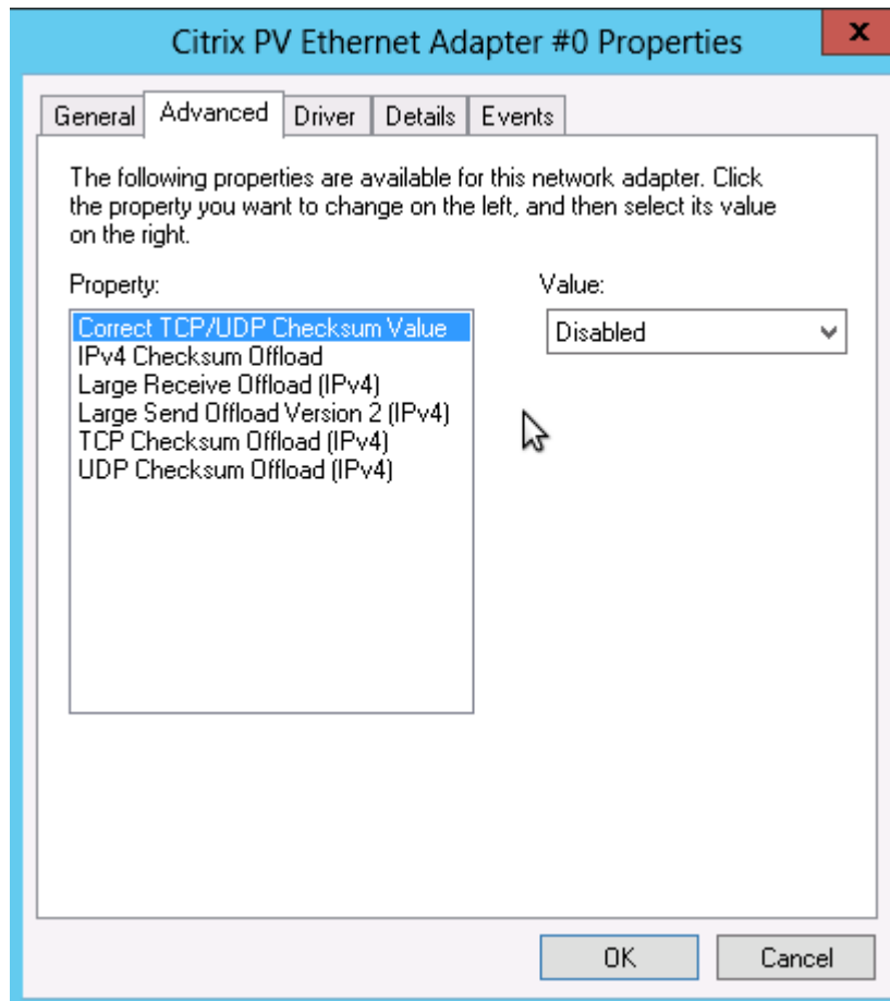
Figure 46 The TCP offload settings for the Citrix adapter
