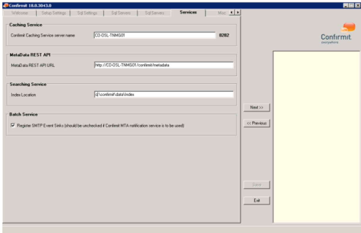
Figure 19 The Services page
